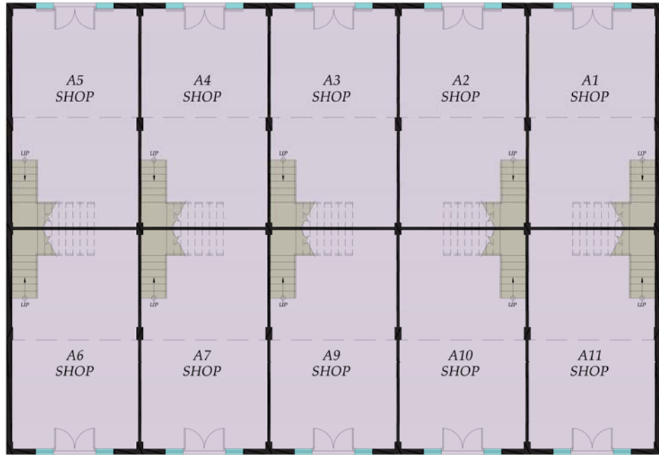
BLOCK-A (GROUND FLOOR PLAN)
