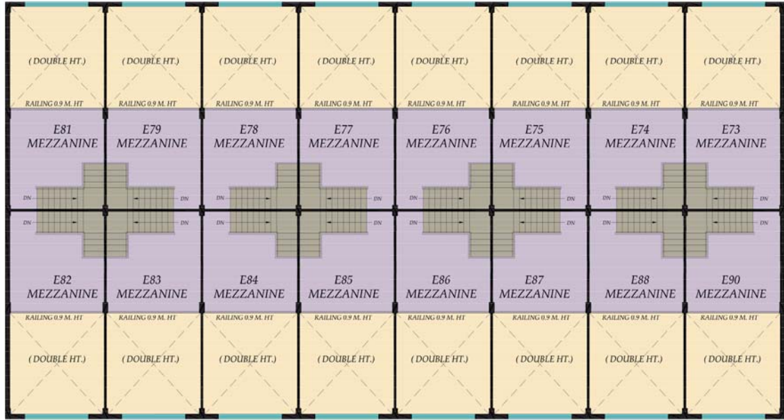
BLOCK-E (MEZZANINE FLOOR PLAN)
