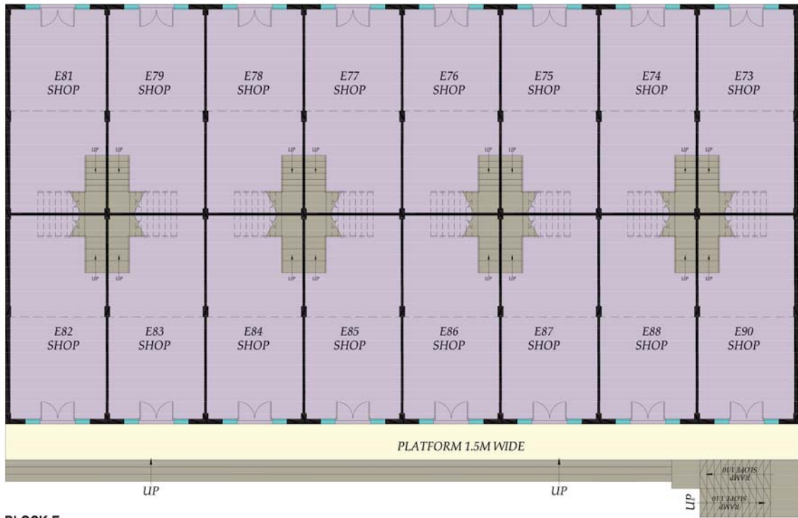
BLOCK-E (GROUND FLOOR PLAN)
