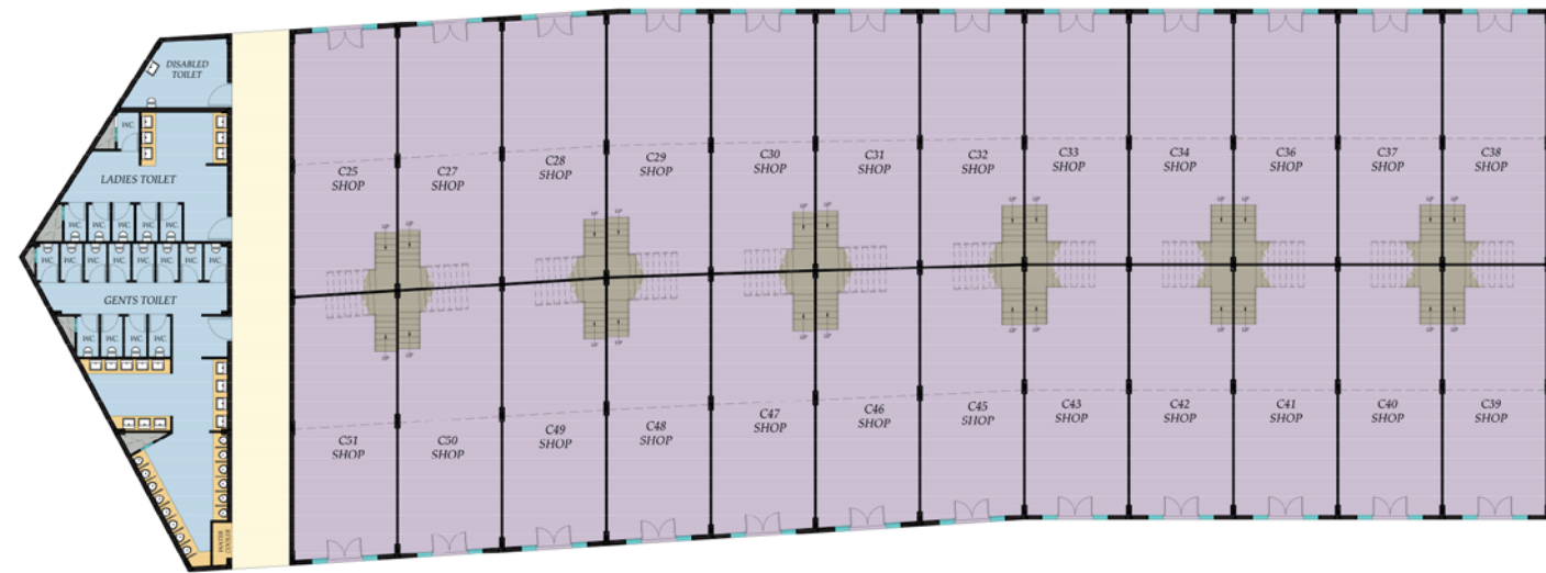
BLOCK-C (GROUND FLOOR PLAN)
